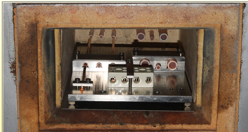
Test oven for the resistivity of ceramics as a function of temperature (Ultimheat Laboratory)
