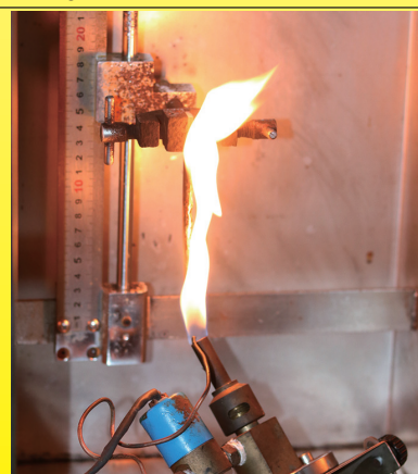
Specimen during UL94VO checking
